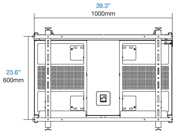
FRONT VIEW LANDSCAPE ADAPTOR VESA 1000mm x 600mm
