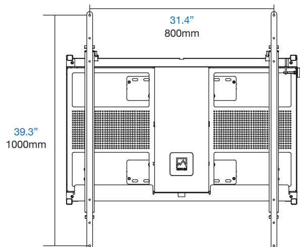
FRONT VIEW PORTRAIT ADAPTOR VESA 800 x 1000mm
